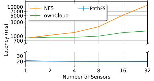
Figure 6: Temperature monitoring average latency.
