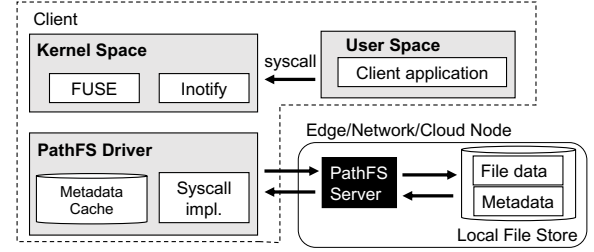
Figure 2: PathFS architecture.
